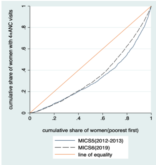
Figure 1 Concentration curves of 4+ANC
